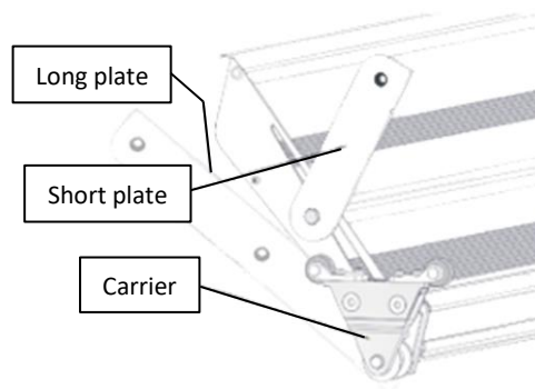
Panel Type 4 – This is the final panel to be placed on the roof
